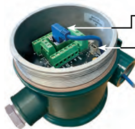
RJ45 Connector for optional Ethernet™ Separate communication channel for SageCom™ diagnostic software via supplied cable or optional Bluetooth® for wireless connectivity to multiple flow meters
